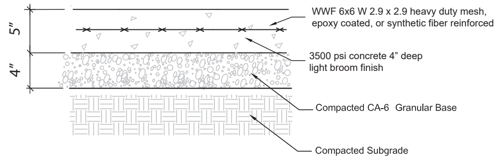
2 PCC Pad Detail (Not to Scale)
