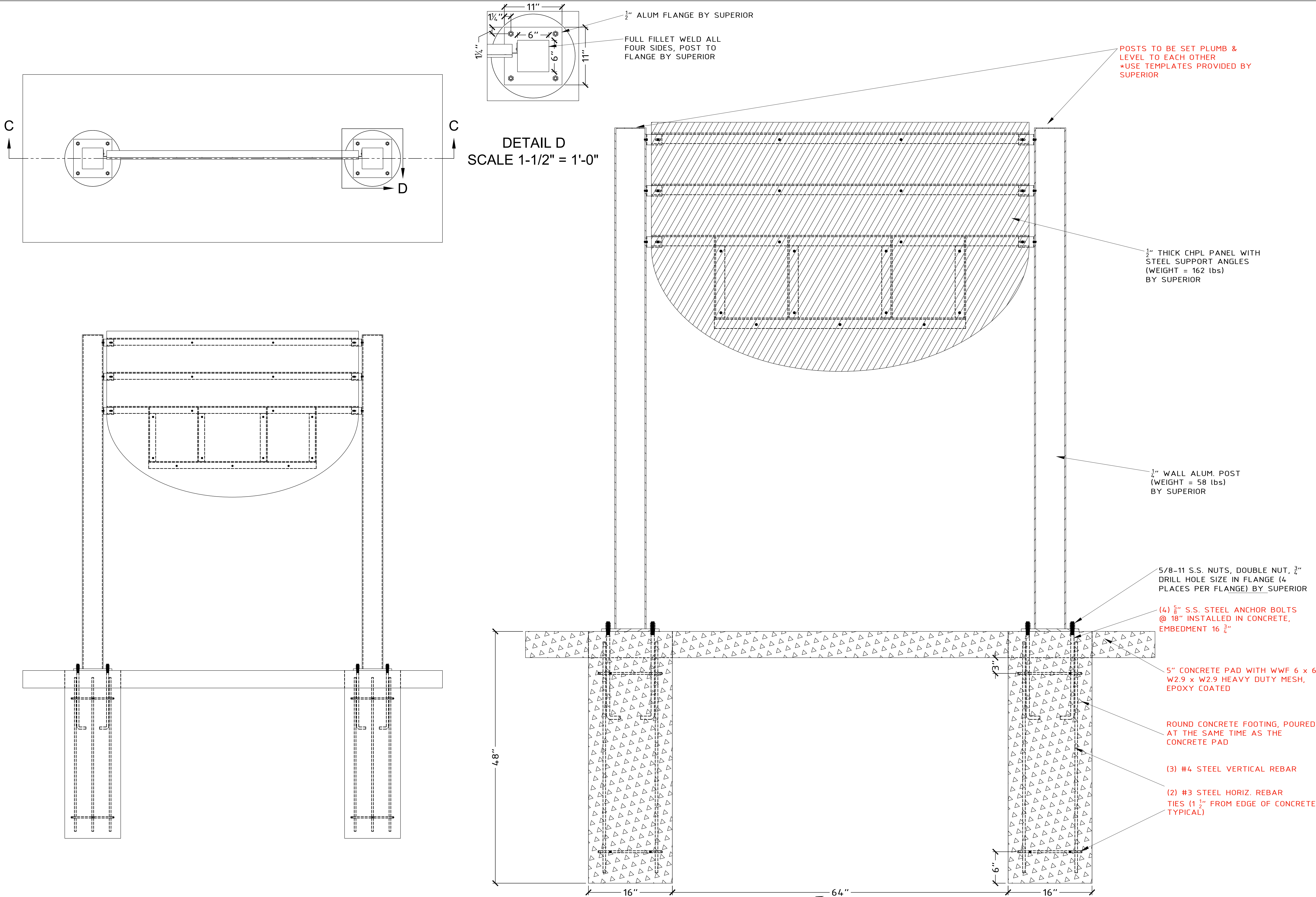
TYPICAL PAD & FOOTING DETAIL FOR ALL KIOSKS WITH 6" POSTS (E-2)
