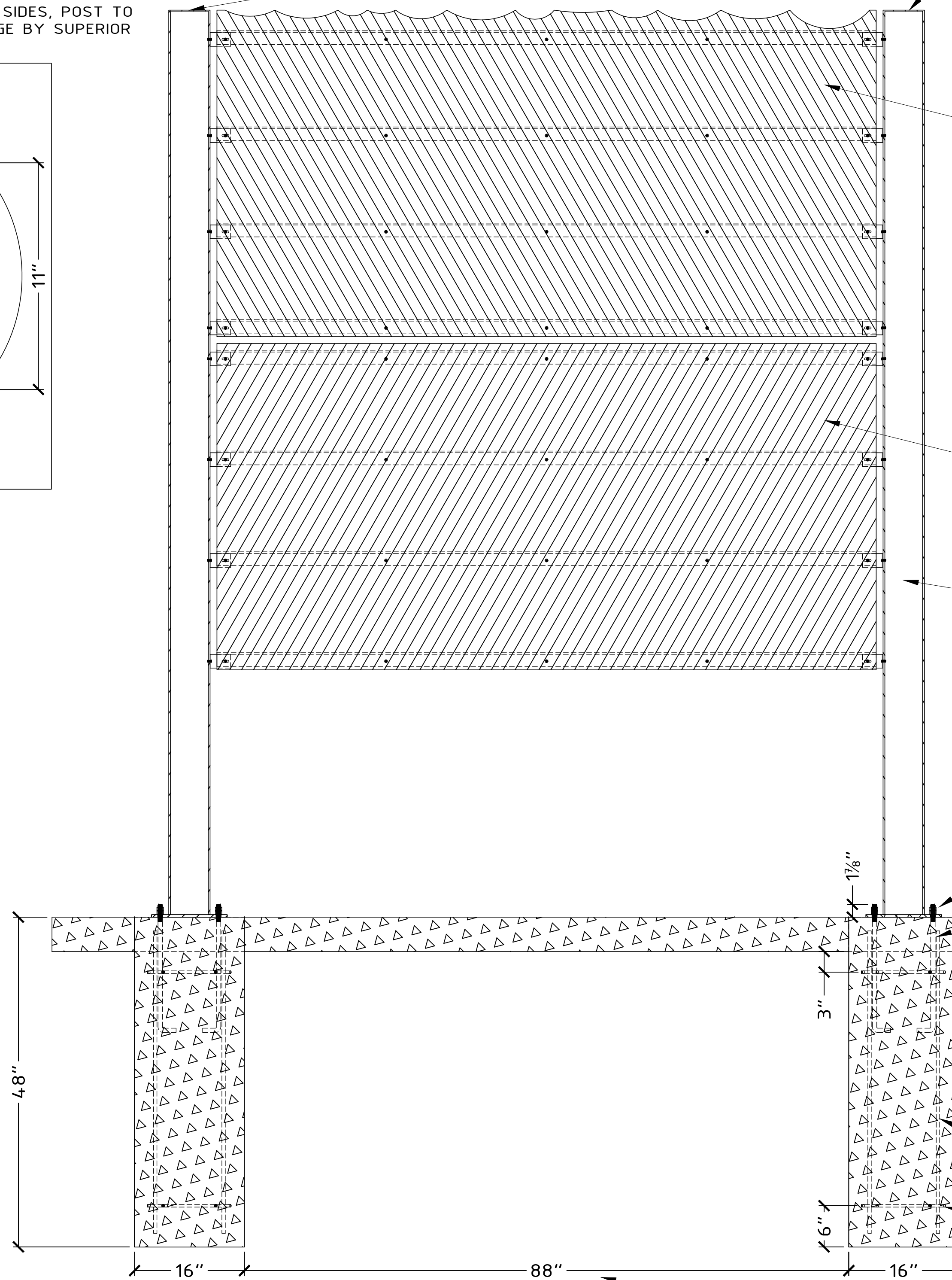
SECTION E-E SCALE 1" = 1'-0"
