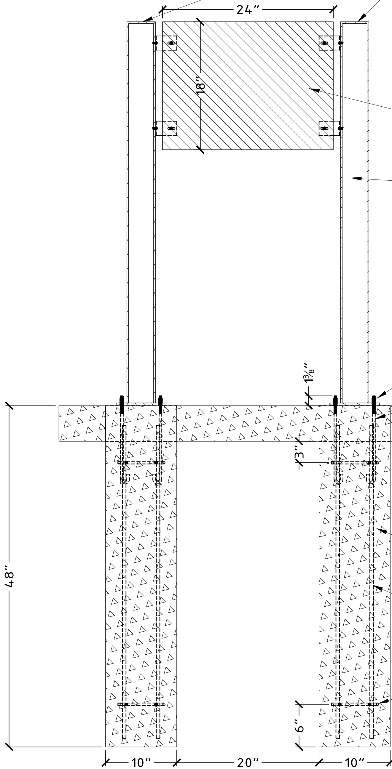
SECTION E-E SCALE 1-1/2" = 1'-0"
