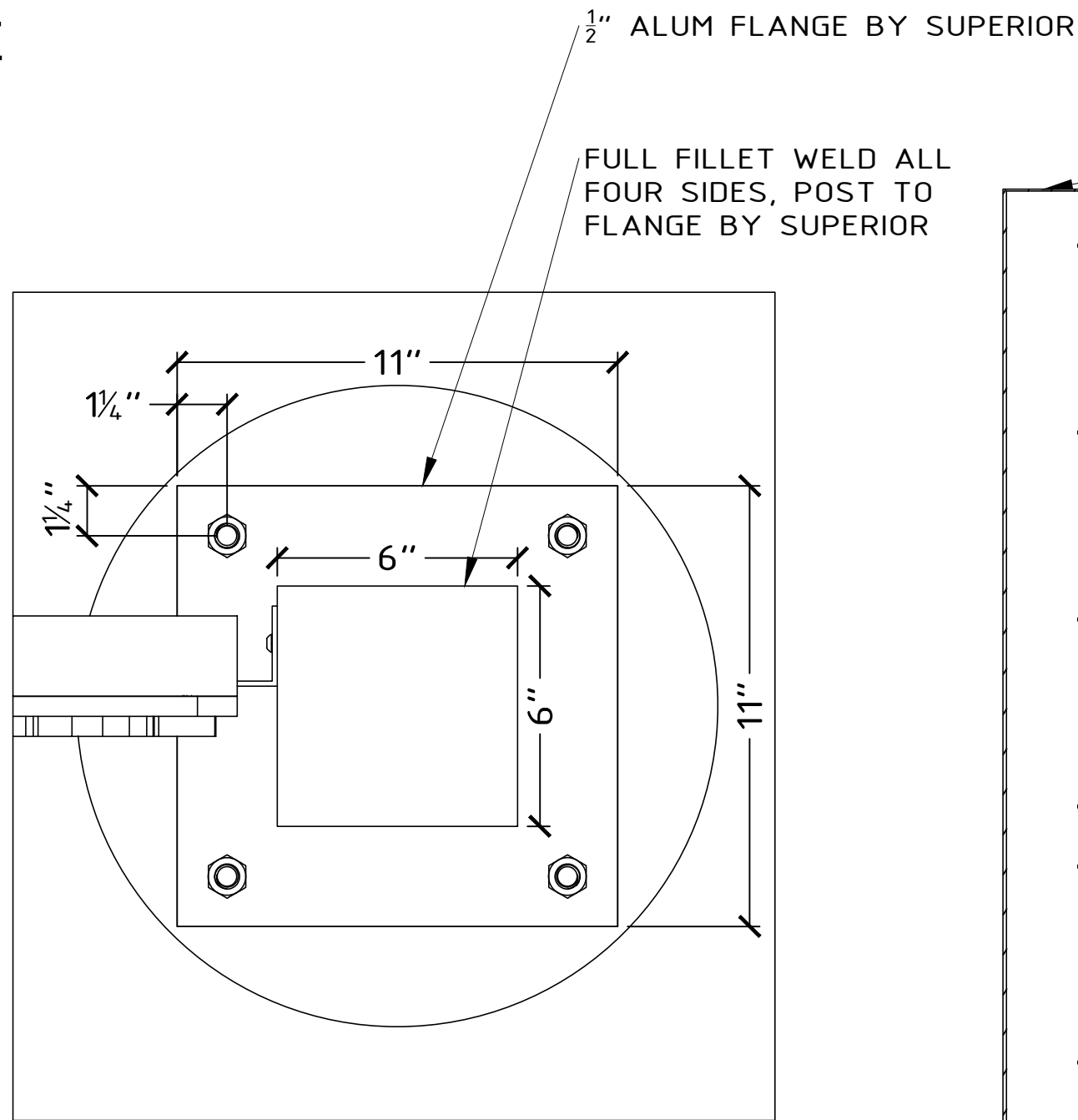
DETAIL F SCALE 3" = 1'-0"
