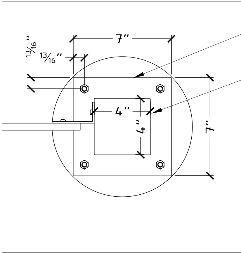
DETAIL F SCALE 3" = 1'-0"
