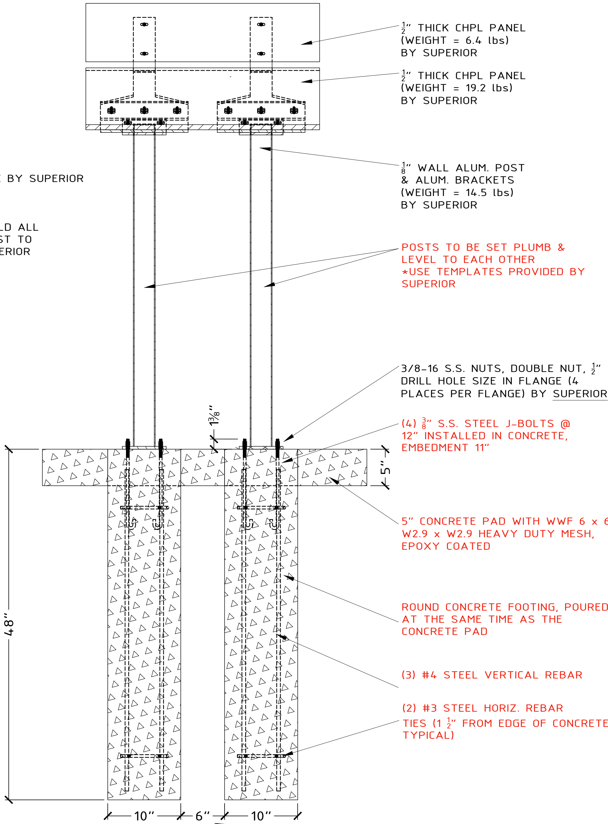
SECTION F-F SCALE 1-1/2" = 1'-0"
